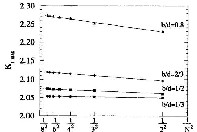
Fig. 3 Relationship between K_{tmax} and 1/N^2 in Fig. 2(b) ( a/b=1.0 , \theta=\pi/2 )
