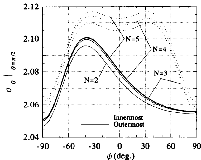
Fig. 8 Distribution of stress at the innermost and outermost cavity in Fig. 2(b) ( a/b=1.0 , b/d=2/3 , \theta=\pi/2 )
